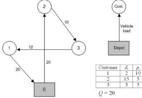
Figure 1: VRPSPD example
