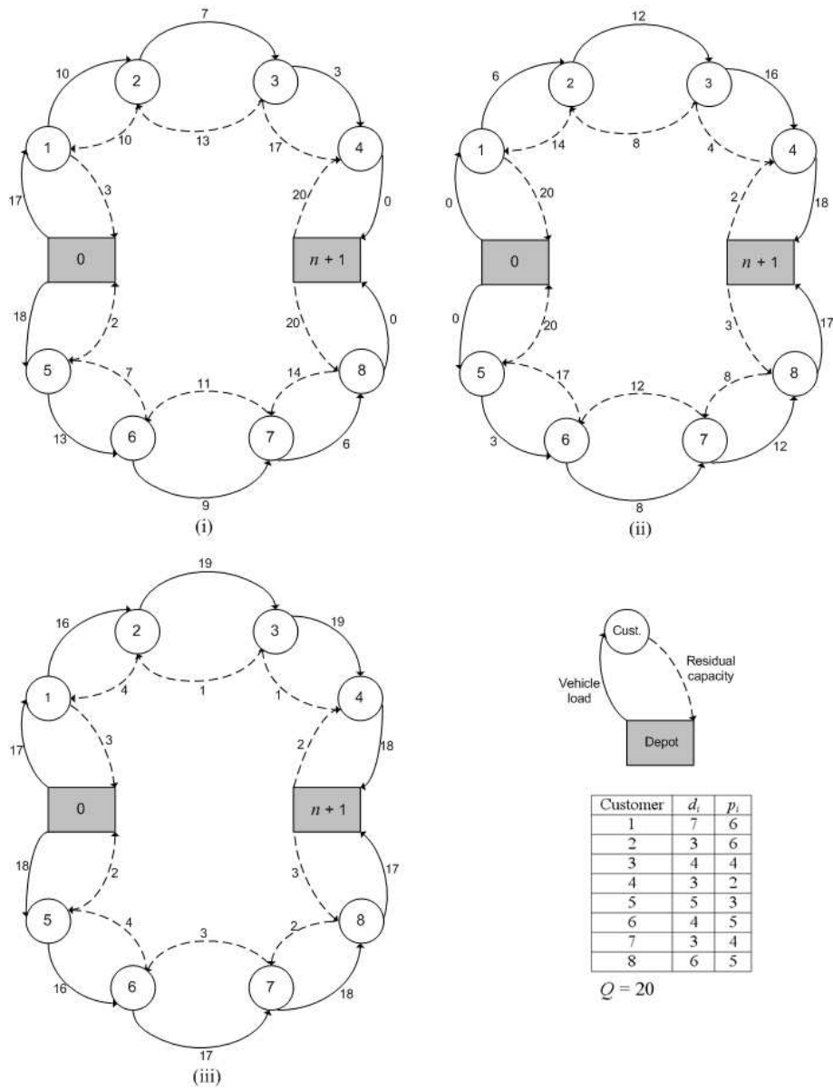
Figure 2: The two-commodity formulation scheme for the VRPSPD
